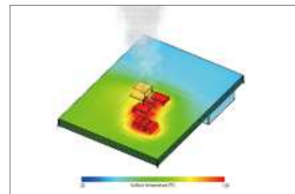
Alert function You can check parts whose temperature is higher than threshold
