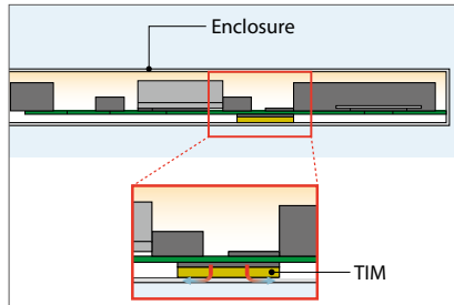
Consideration of simple enclosure You can consider heat dissipation by connection to enclosure
